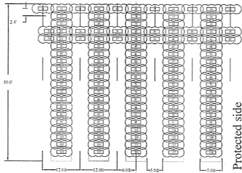
FIG. 8. Layout of DMM columns, Orleans Avenue Canal, New Orleans (Woodward, 2006).
