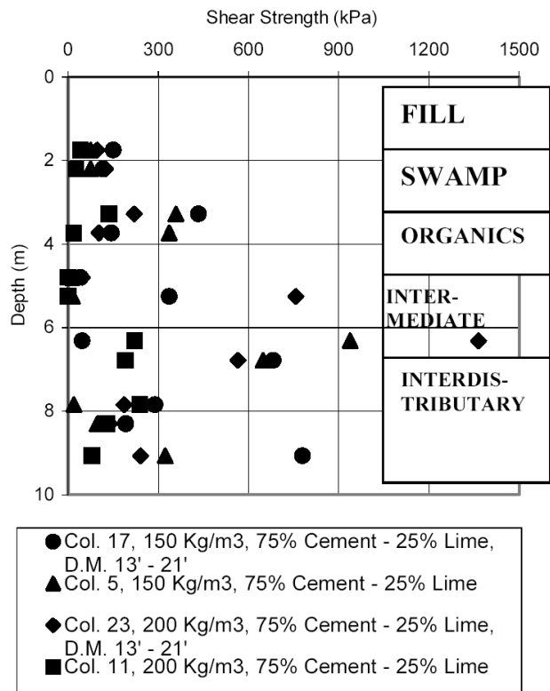
FIG. 3. Shear test results on core samples.
