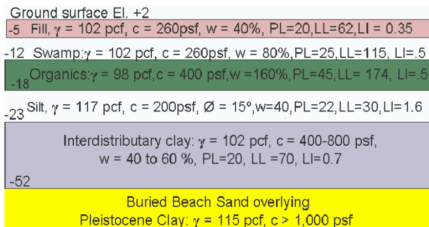
FIG. 2. Generalized site stratigraphy and soil properties.
