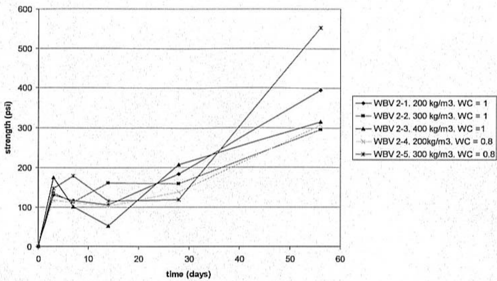
FIG. 6. Westwego Pump Station, 56-day bench scale results at 28 to 80 feet (Woodward, 2008).
