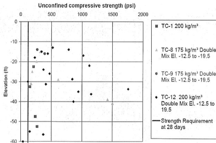
FIG. 11. Unconfined compressive strength results of in-situ test columns, 17 th Avenue Canal, New Orleans.
