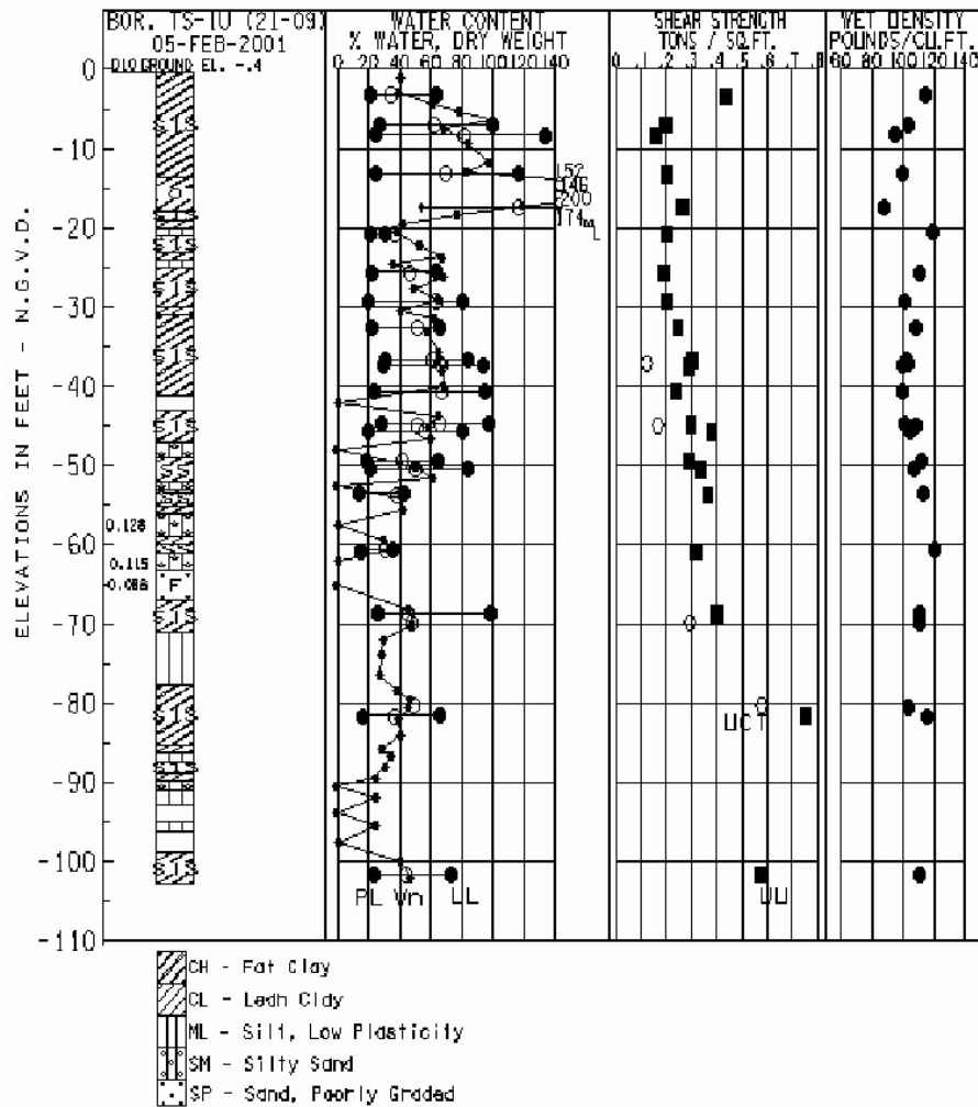
FIG. 1. Soil properties from one 5-inch diameter, undisturbed boring.
