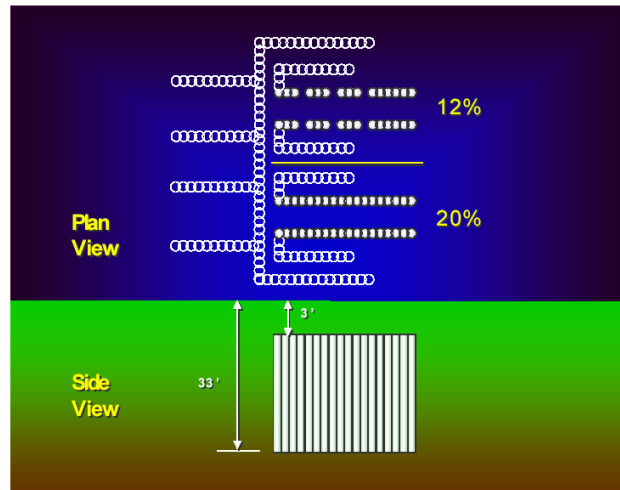
FIG. 4. As-built cell configuration with 12% and 20% replacement ratios.
