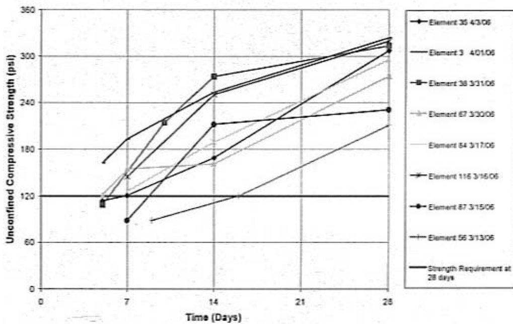
FIG. 9. Wet grab sample results, upper 10 feet, Orleans Avenue, New Orleans.
