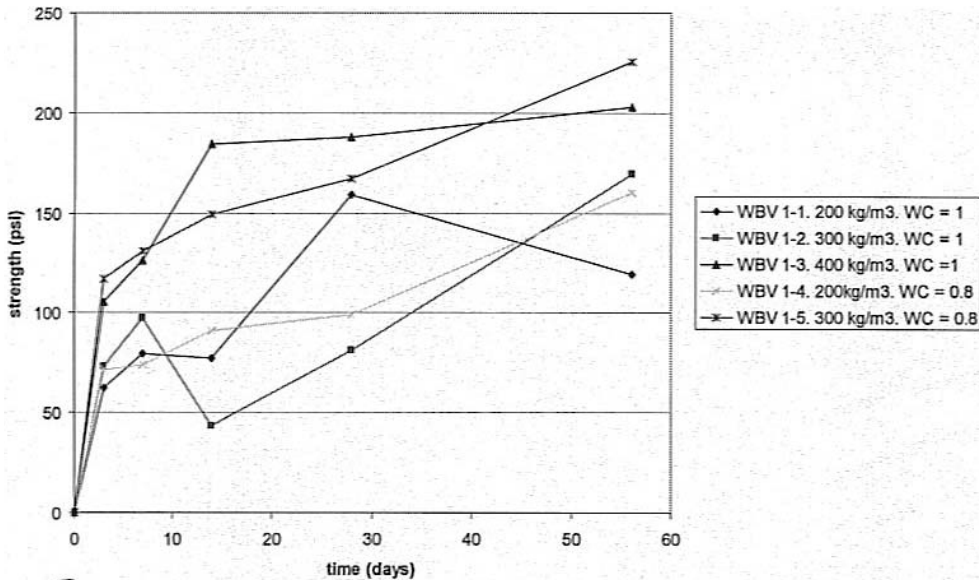
FIG. 5. Westwego Pump Station, 56-day bench scale results of the upper 25 feet (Woodward, 2008).
