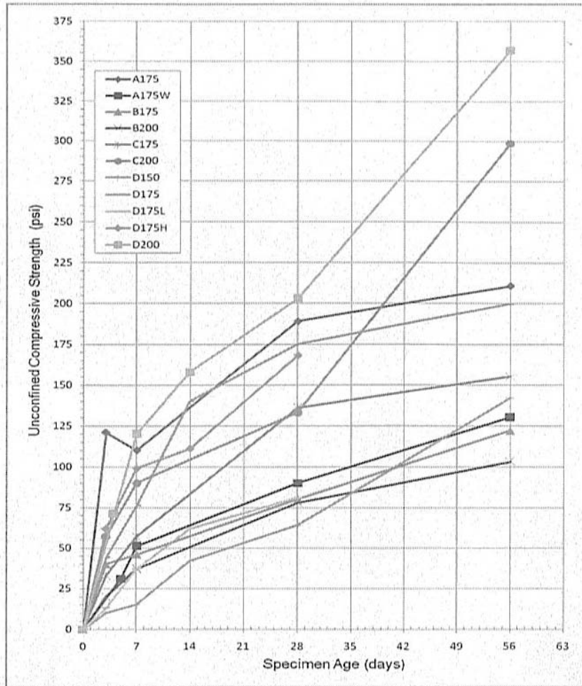
FIG. 7. Bench scale test results, Plaquemines Parish Homeplace Levee Setback (Woodward, 2006).
