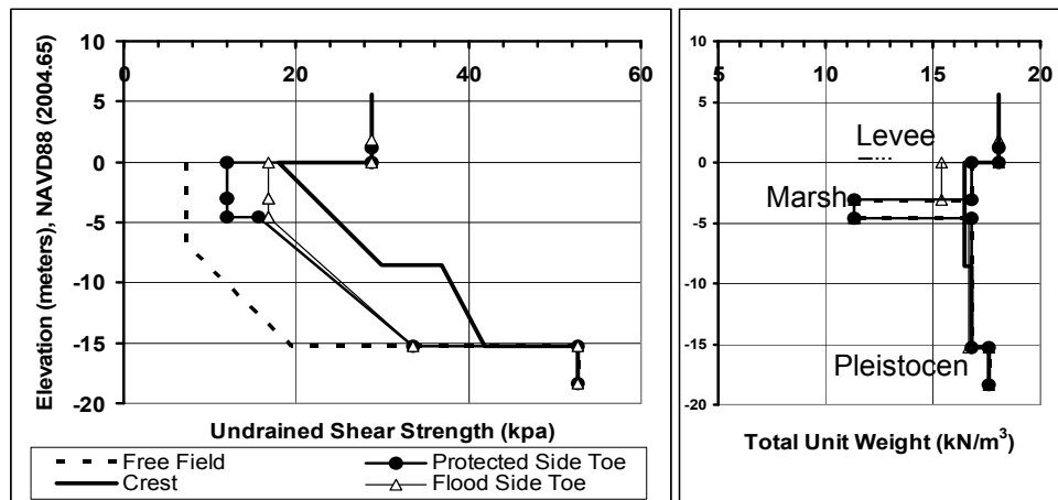
FIG. 12. Design undrained shear strength and total unit weight, reach 12B (Cooling et al., 2012).
