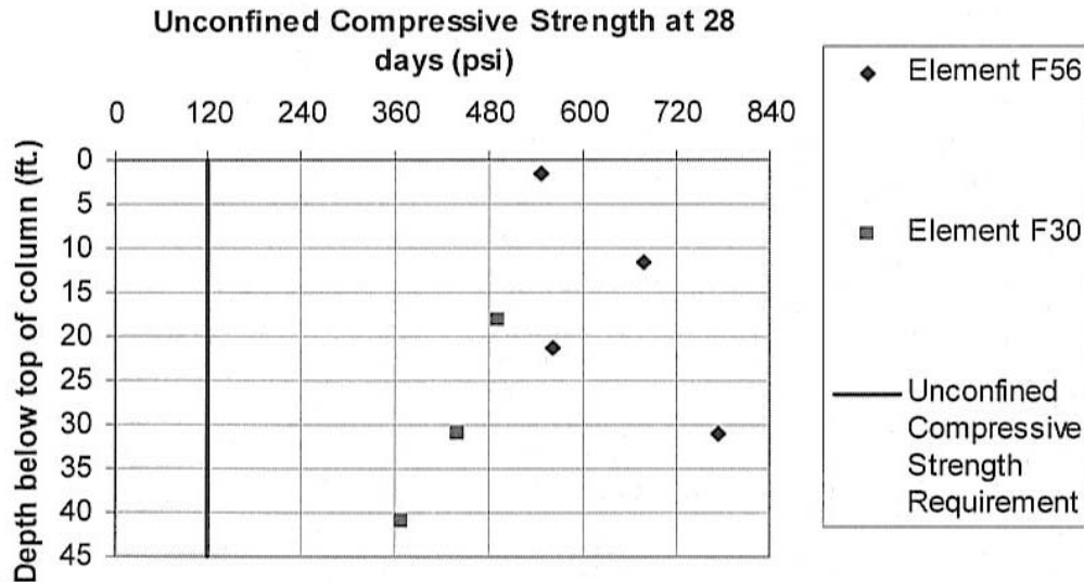
FIG. 10. Orleans Avenue, in-situ column coring results at 28 days (Woodward, 2006).
